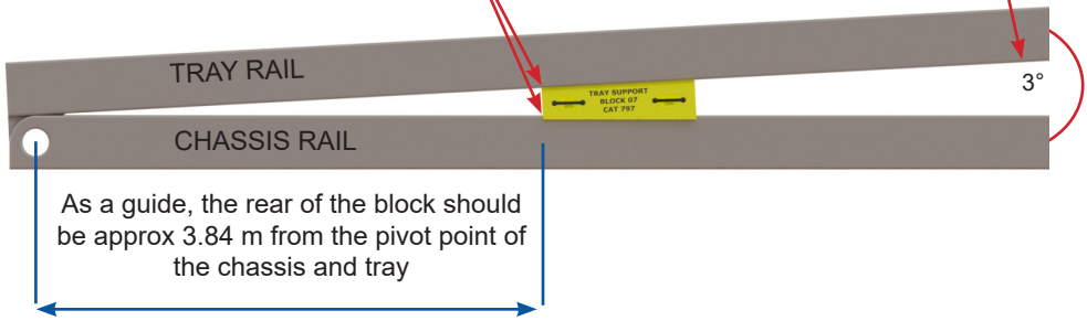
Tray rail contact area
